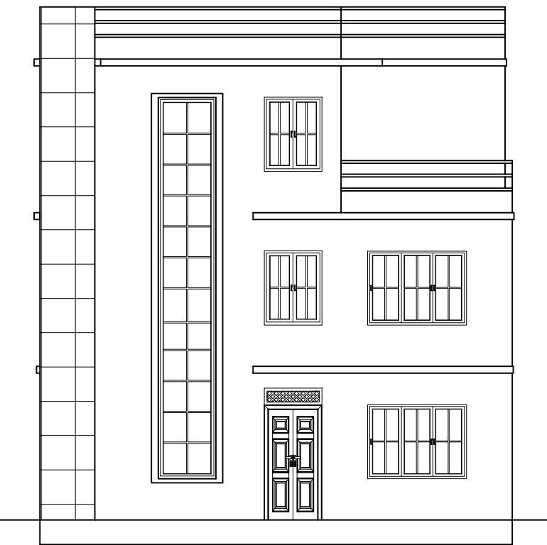
SOUTH ELEVATION
