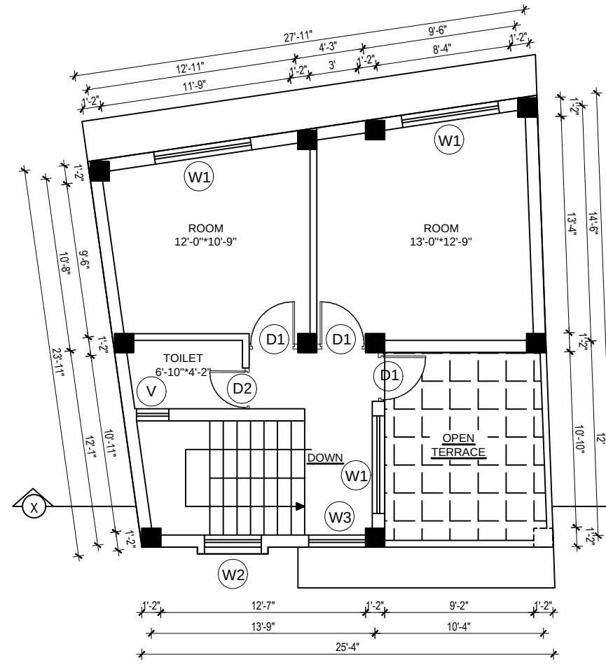
SECOND FLOOR PLAN AREA : 566.08 SQ. FT.
