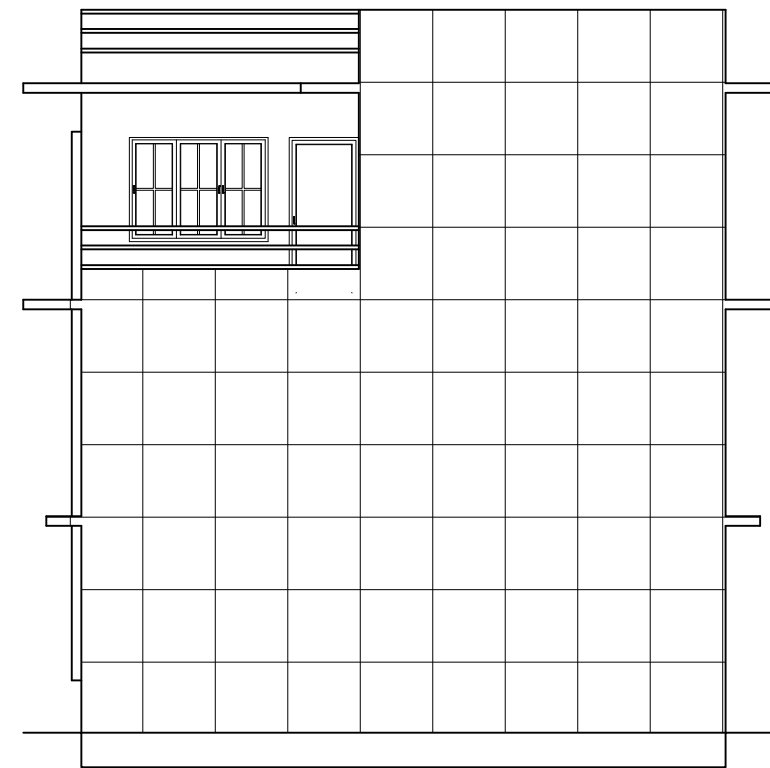
EAST ELEVATION
