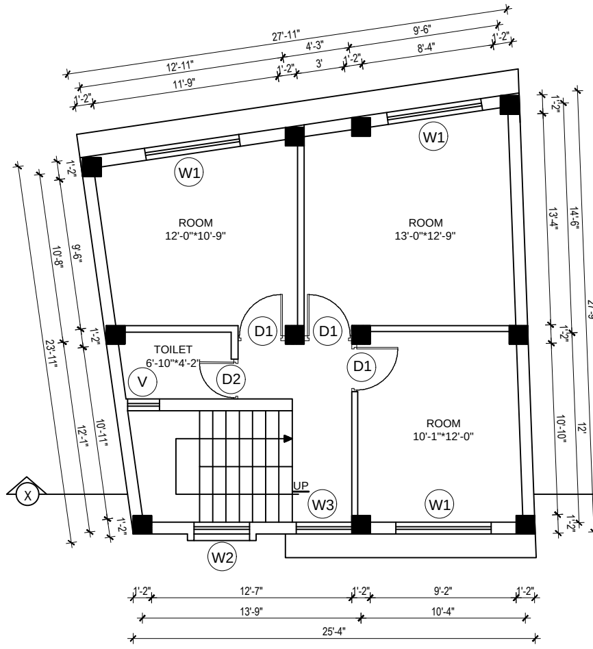
FIRST FLOOR PLAN AREA : 687.75 SQ. FT.
