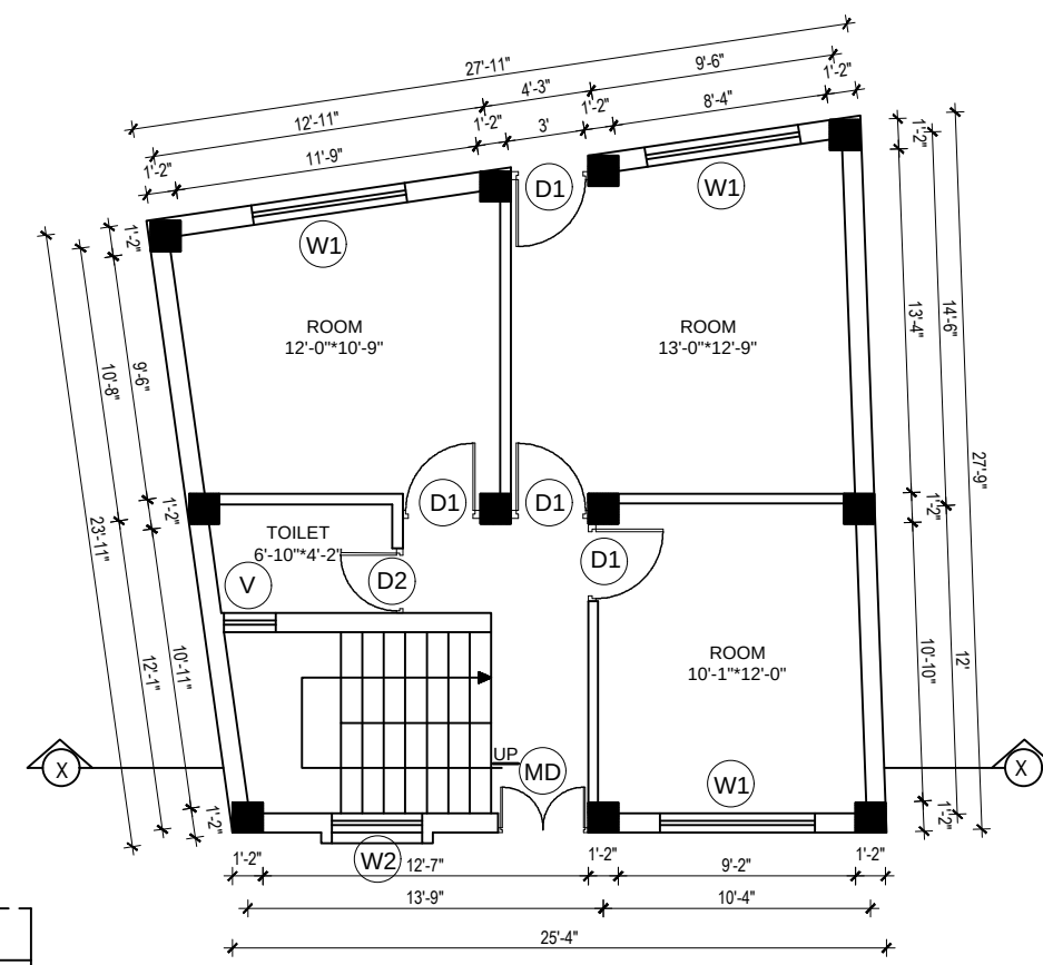
GROUND FLOOR PLAN AREA : 687.75 SQ. FT.
